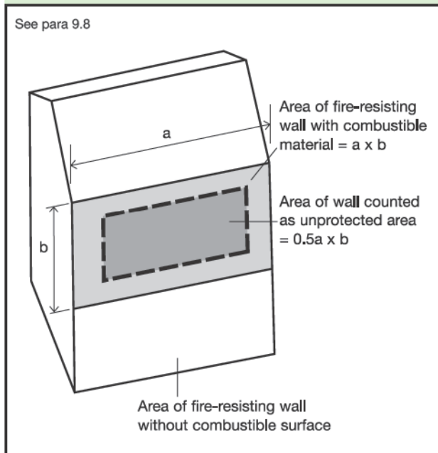
Diagram 19 Status of combustible surface material as unprotected area
