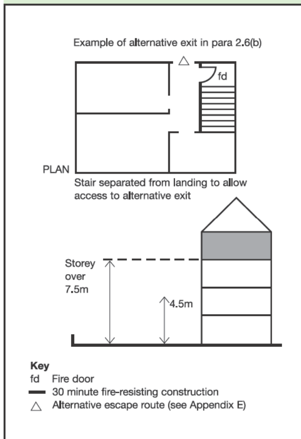
Diagram 3 Fire separation in houses with more than one floor over 4.5m above ground level
