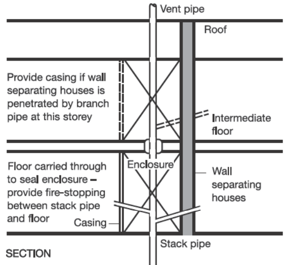
Diagram 15 Enclosure for drainage or water supply pipes
