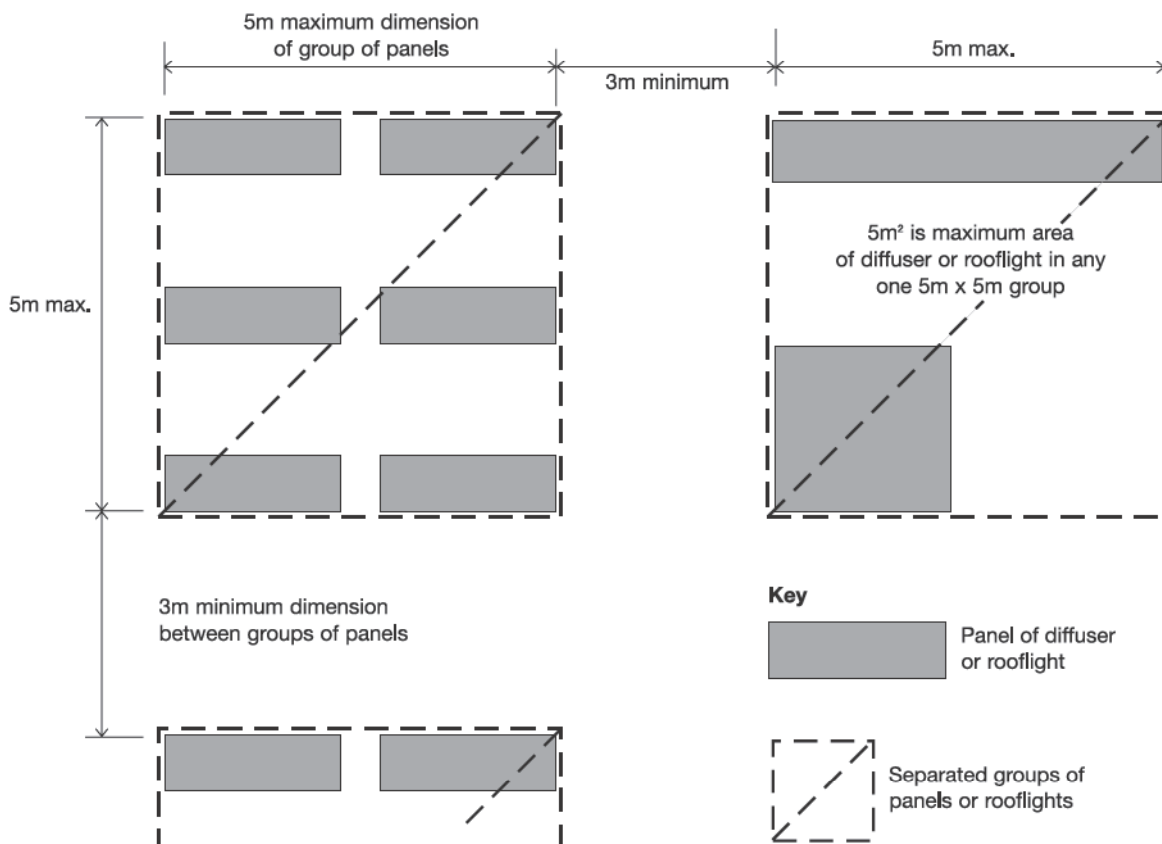
Diagram 9 Layout restrictions on Class 3 plastic rooflights, TP(b) rooflights and TP(b) lighting diffusers
